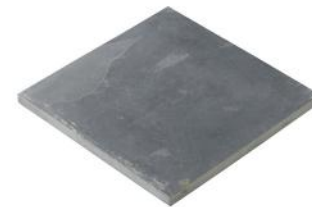
Black Slate
